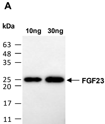
Fig 1. Western blot of recombinant human FGF23 protein (A, 10 ng; B, 30 ng), using Ab (M0010-1-TC) at RT for 2 h.
